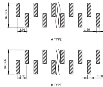
Recommended P.C.B Layout(Top Side) (PCB BOARD TOLERANCE±0.05)
